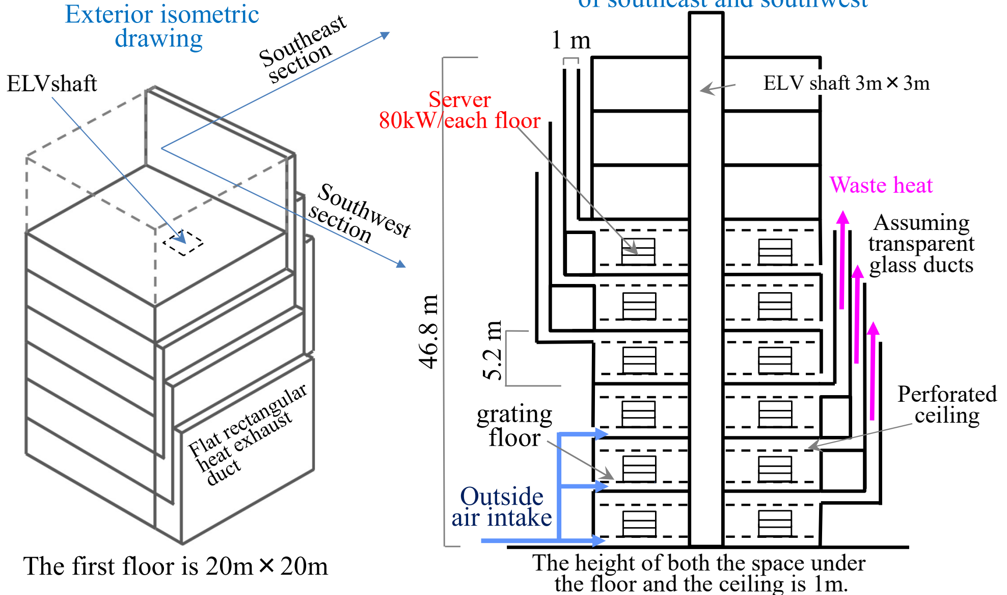
Schematic diagram of composite cross section of southeast and southwest
